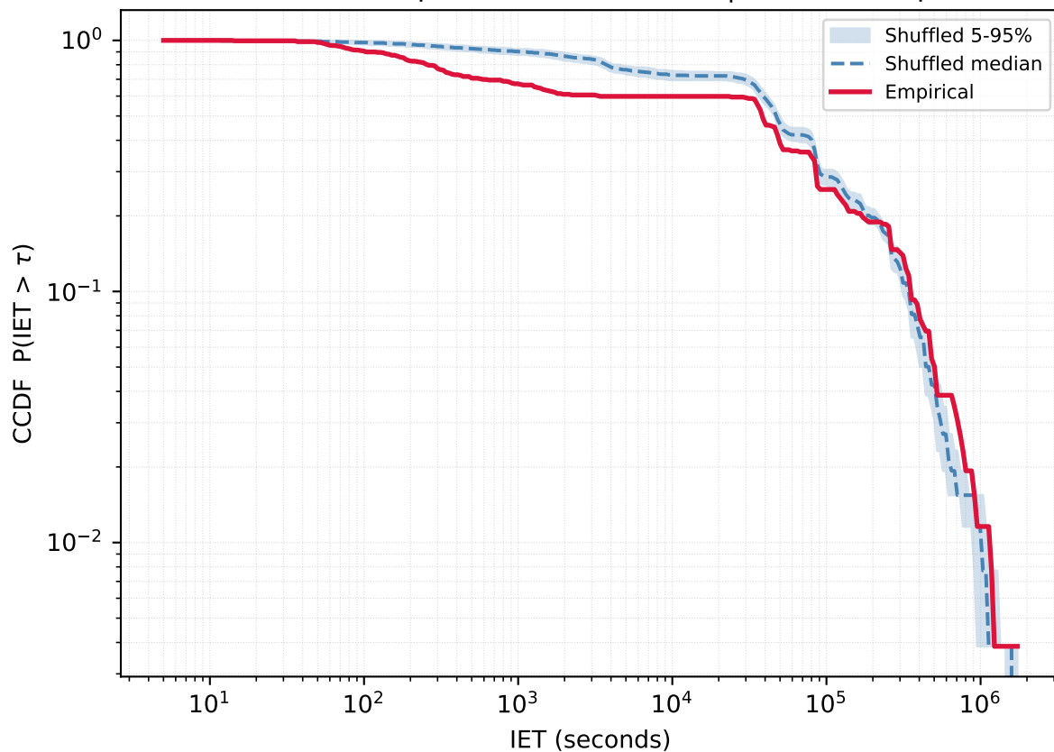
User 8786749 - Empirical vs Reshuffled | KS=0.261 p=0.000
